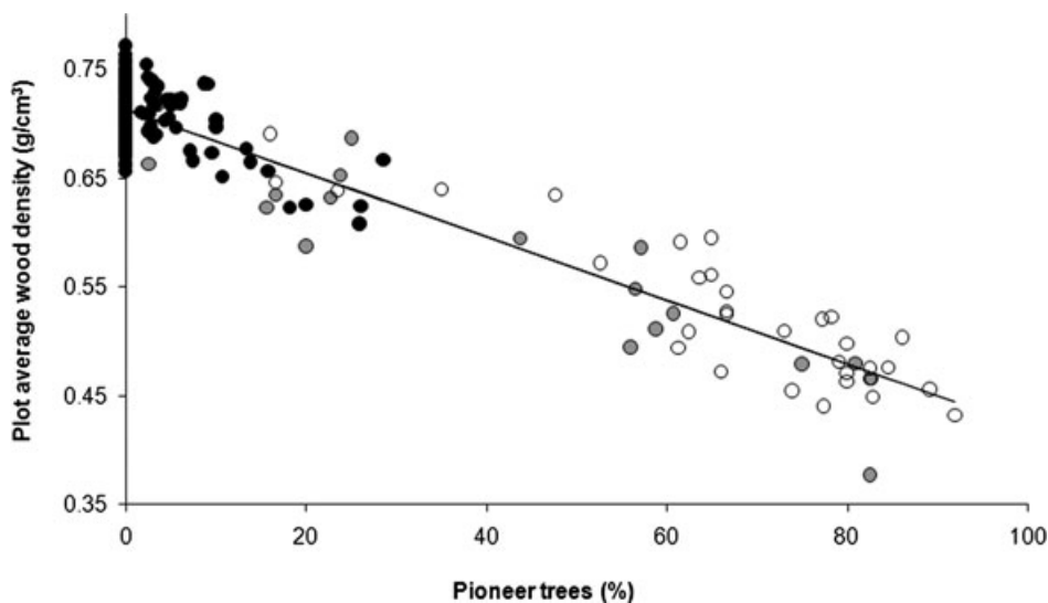
Figure 2. Relationship between average air-dried wood density and percentage of pioneer trees in 159 plots of 0.01 \text{ ha} in the local Samboja-Sungai Wain data set (correlation coefficient of -0.95 , R^2 of 90.3\% , df = 158 , p < 0.0001 ; undisturbed plots, black dots; once-burned plots, gray dots; twice-burned forest, open dots).
